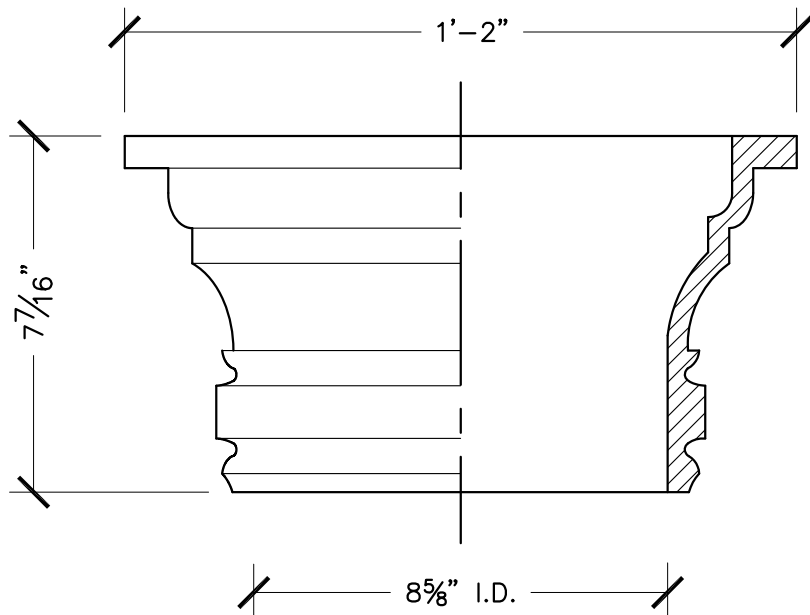
ELEVATION / SECTION
